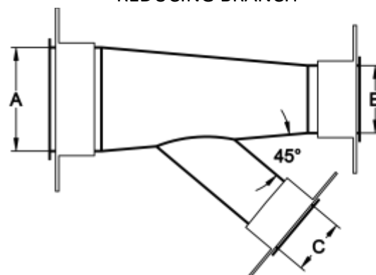
REDUCING BRANCH
