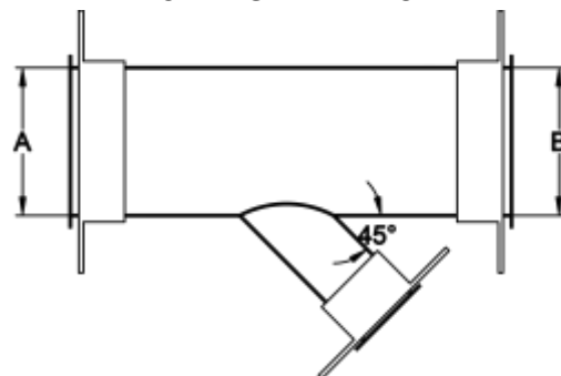
STRAIGHT BRANCH
